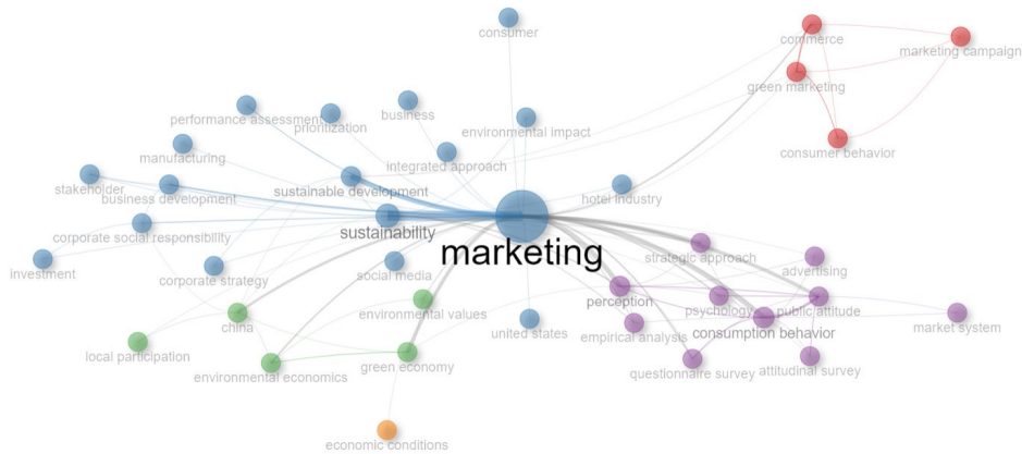
Figure 7. Co-occurrence network
